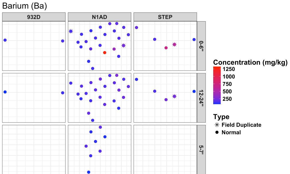
Figure D-3.1 Concentrations of barium (mg/kg) at each soil sampling location, displayed by the northing and easting relative to an origin for the NAD 1983 State Plane system for Montana.
