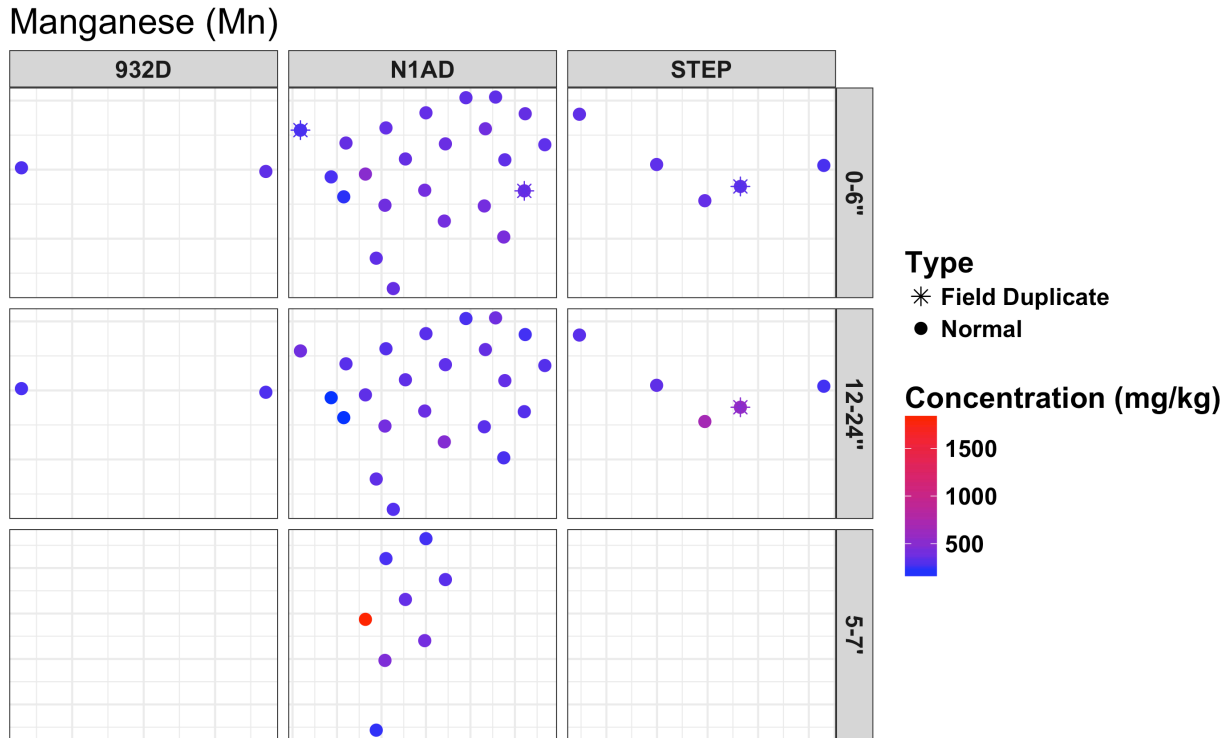
Figure D-3.5. Concentrations of manganese (mg/kg) at each soil sampling location, displayed by the northing and easting relative to an origin for the NAD 1983 State Plane system for Montana. The top plot is paneled by depth only, and the bottom plot is paneled by depth and area to zoom in on each sampling area.
